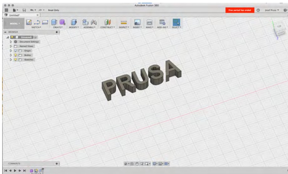
Obr. 26 - Fusion 360
